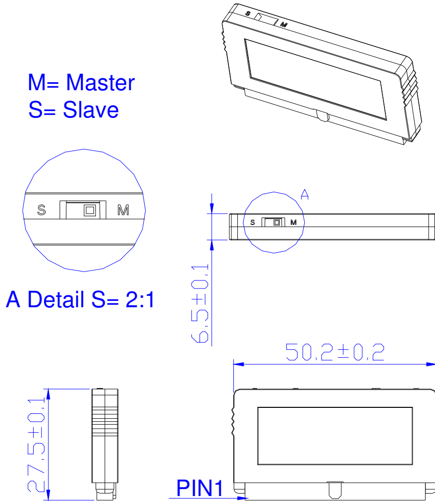
Figure 2: DOM Dimensions
